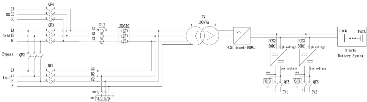
Figure 1-2 Electrical Wiring Diagram
